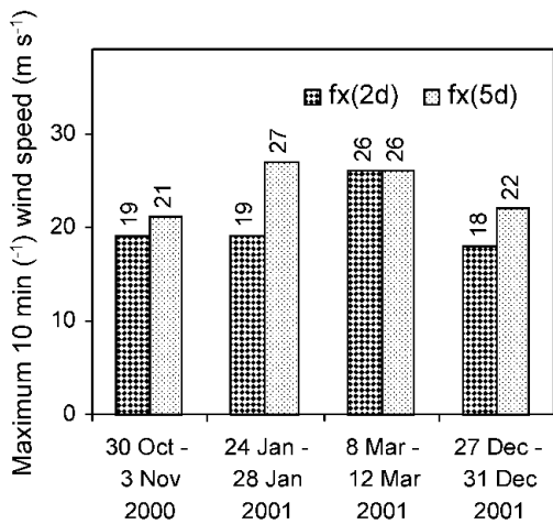
Fig. 5. The maximum 10 min wind speed for 2 days, fx(2d) , and 5 days, fx(5d) , at Þverfall before the avalanche days which the models missed (NA in Fig. 3).
