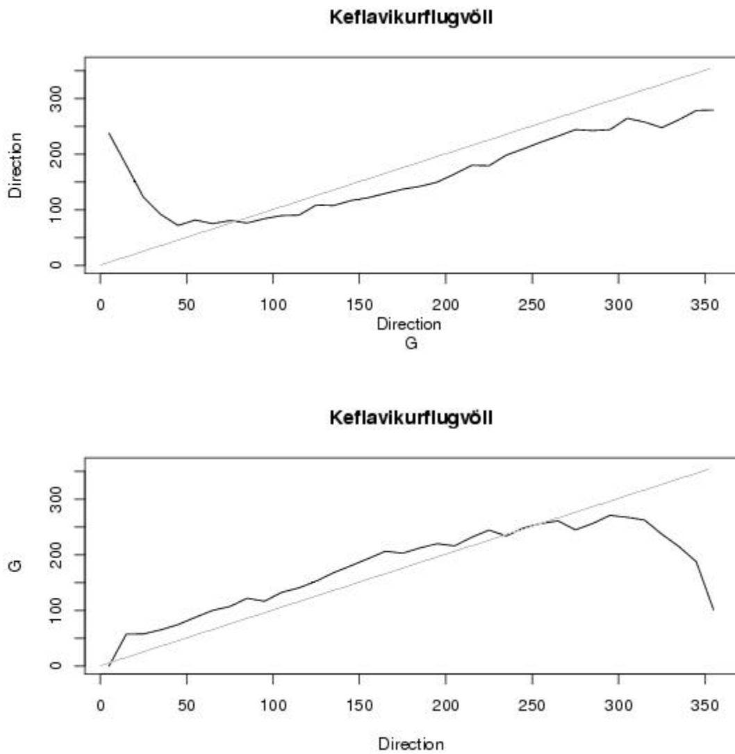
Figure 3 : Observed wind direction at 10 m height vs. the direction of the geostrophic wind at Keflavikurflugvöllur
